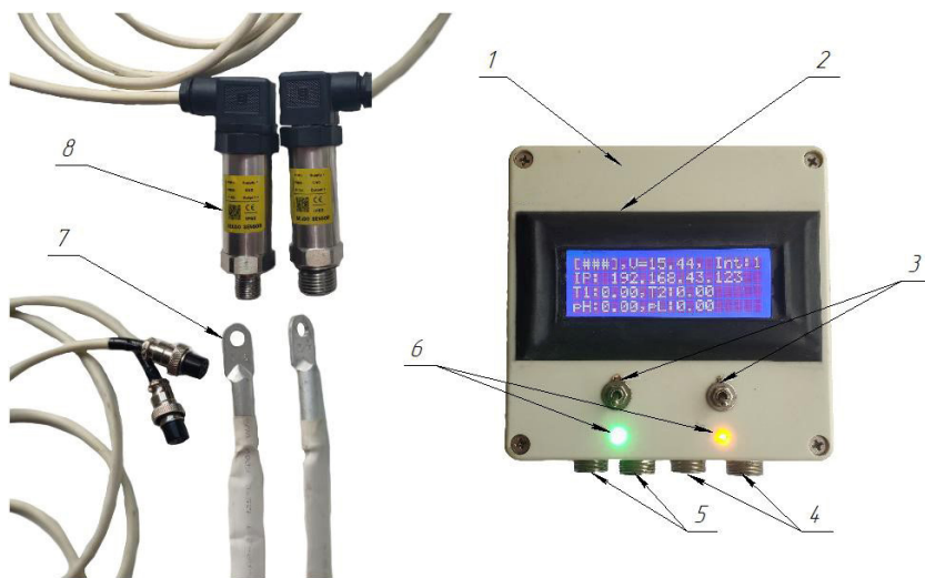
Figure 2. Appearance of the device for measuring the pressure and temperature of the working fluid: 1 – computing unit, 2 – display, 3 – toggle switches, 4 – temperature sensor ports, 5 – pressure sensor ports, 6 – workflow indicators, 7 – temperature sensors, 8 – pressure sensors
